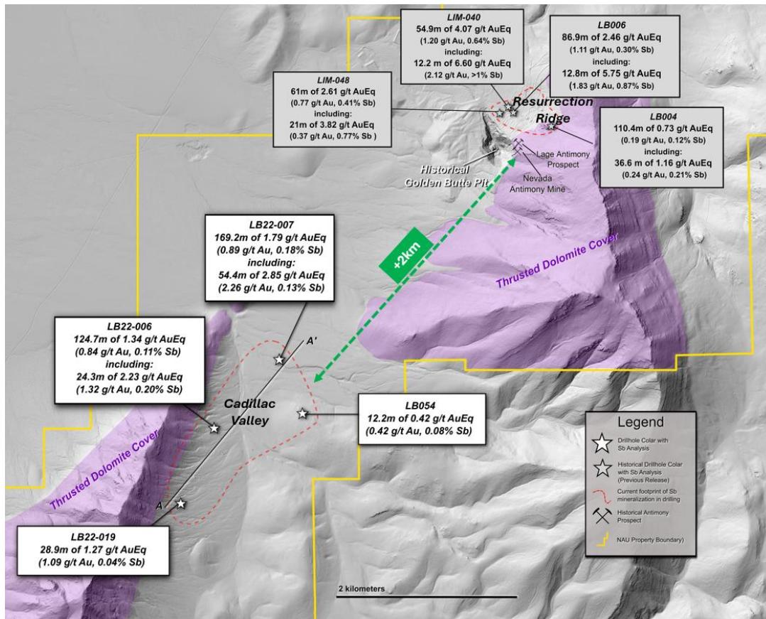
Figure 1 – Limousine Butte Gold-Antimony Project with selected gold-antimony drillhole results.
