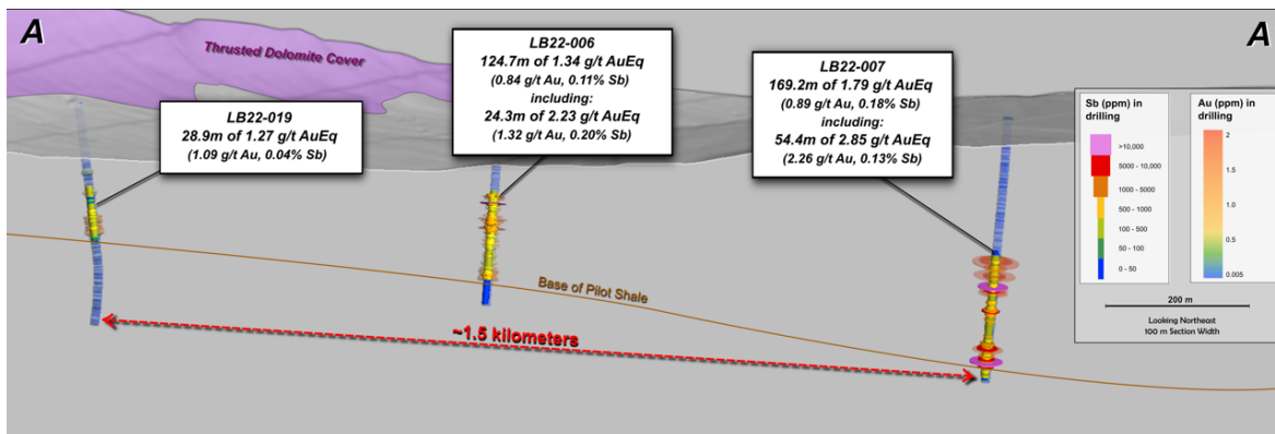
Figure 2 – Limousine Butte Gold-Antimony Project cross-section with selected gold-antimony drillhole results. Thin colored discs show Antimony (Sb ppm) in drilling, and wide colored discs show Gold (Au ppm) in drilling.
